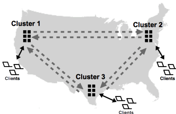
Figure 11.1. Active(N) Cross Datacenter Replication
