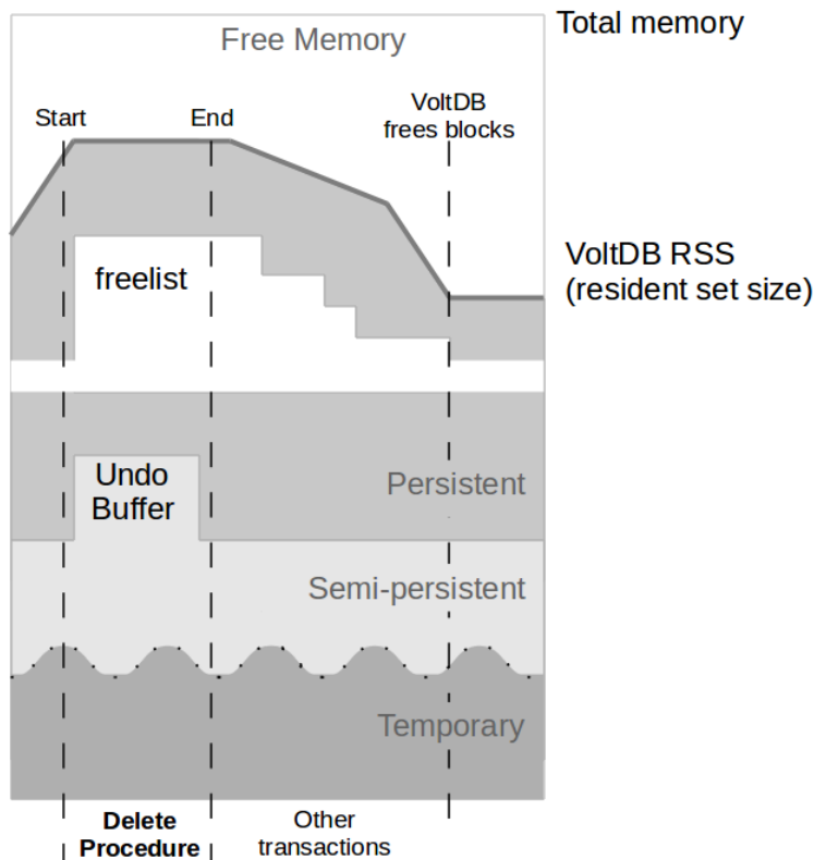
Figure 13.2. Details of Memory Usage During and After an SQL Statement
