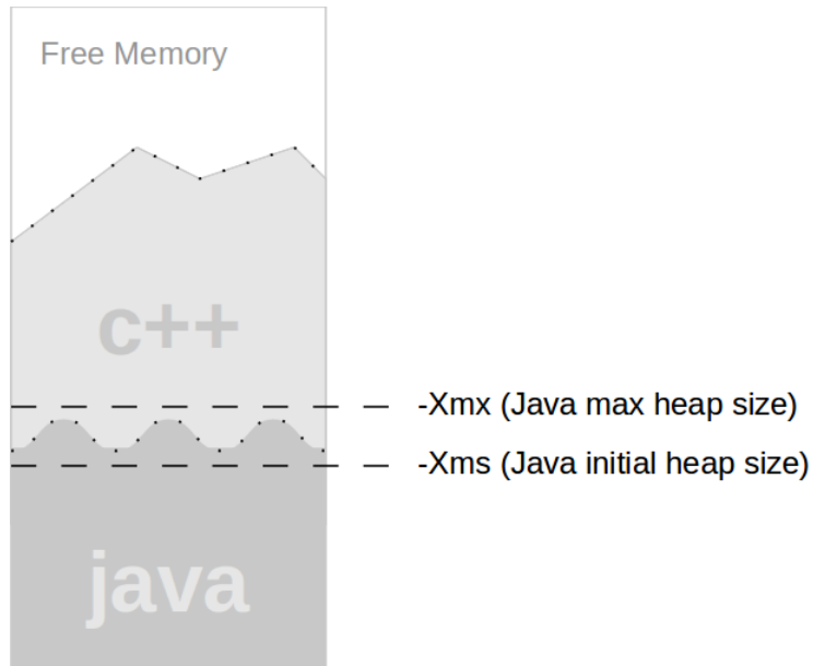
Figure 11.3. Controlling the Java Heap Size
