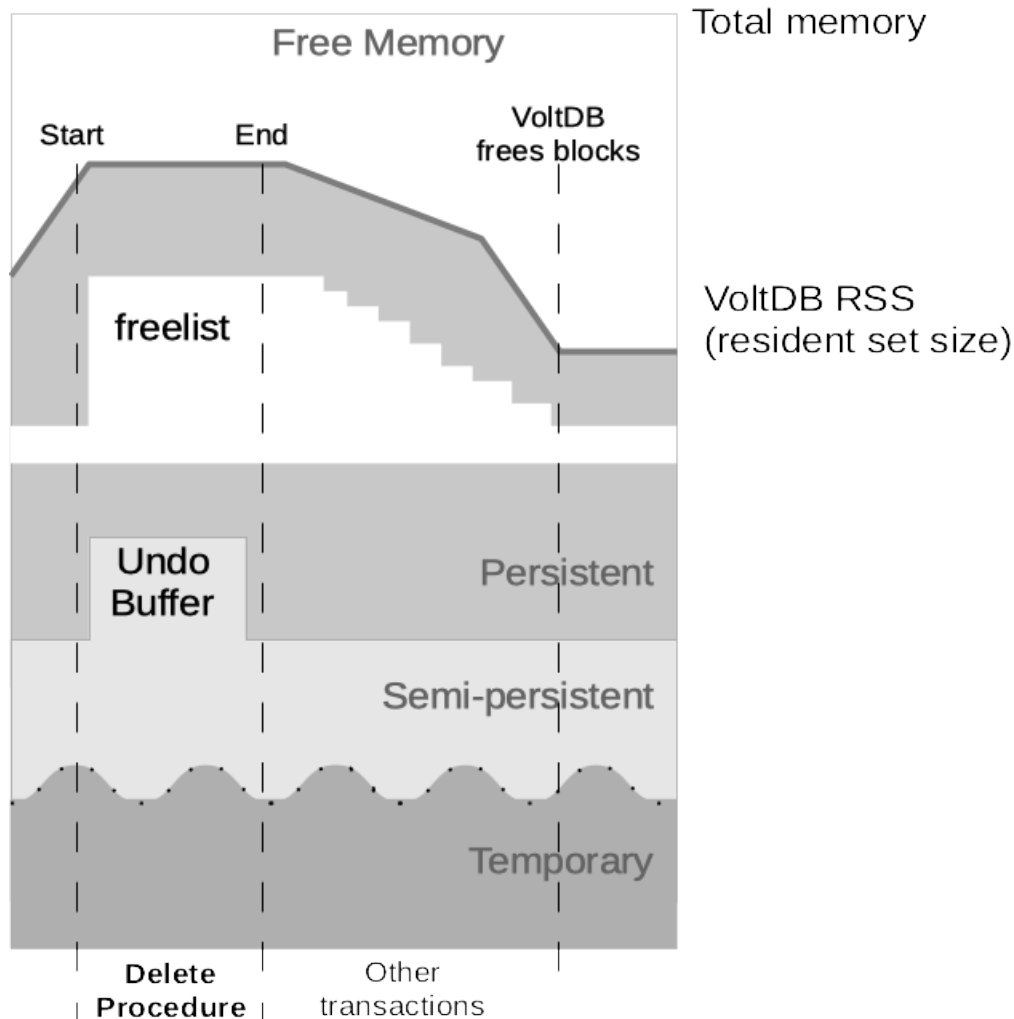
Figure 11.2. Details of Memory Usage During and After an SQL Statement
