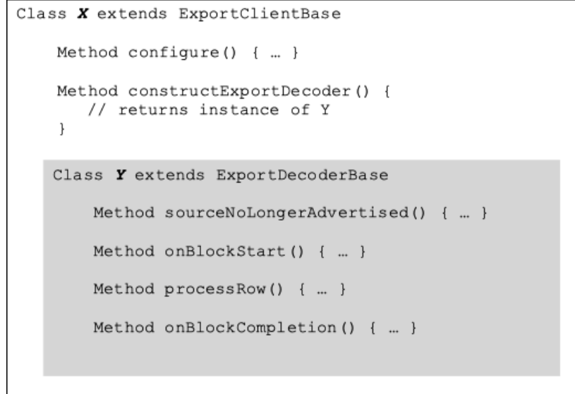
Figure 8.1. Structure of the Custom Export Class
