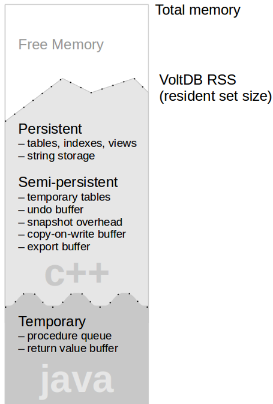
Figure 11.1. The Three Types of Memory in VoltDB
