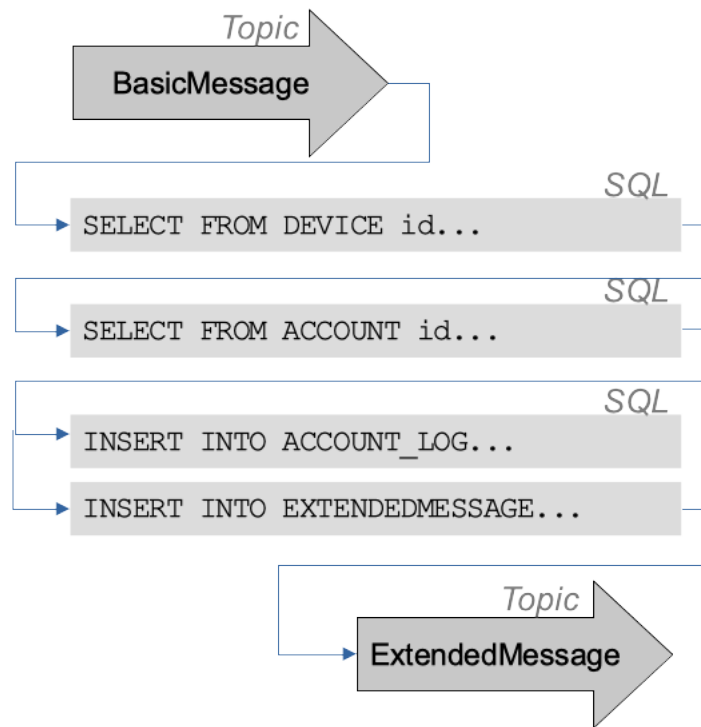
Figure 10.1. Business Logic for Processing Device Messages
